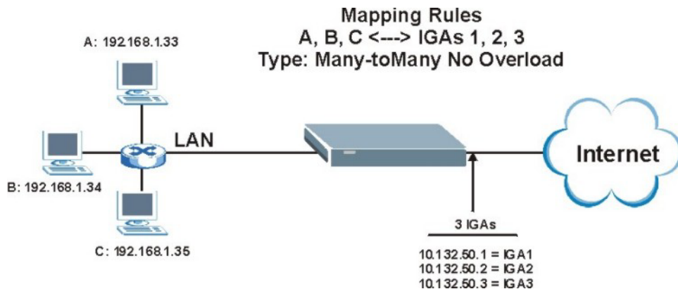
Figure 30-19 NAT Example 4
