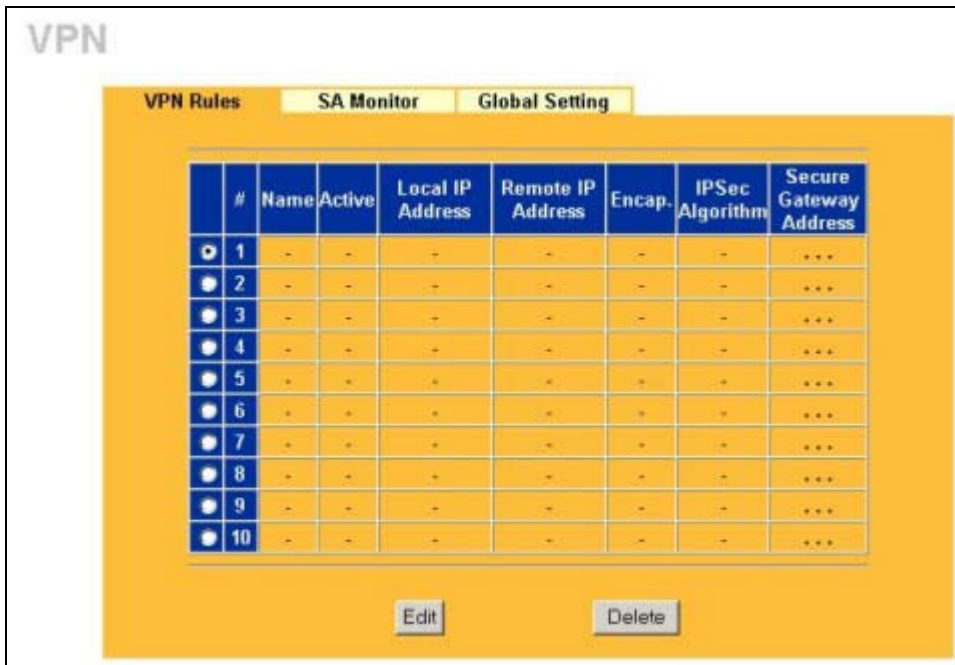
Figure 15-2 VPN Rules
