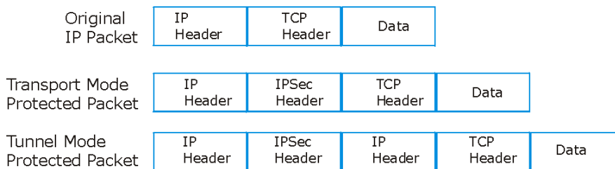
Figure 14-3 Transport and Tunnel Mode IPsec Encapsulation
