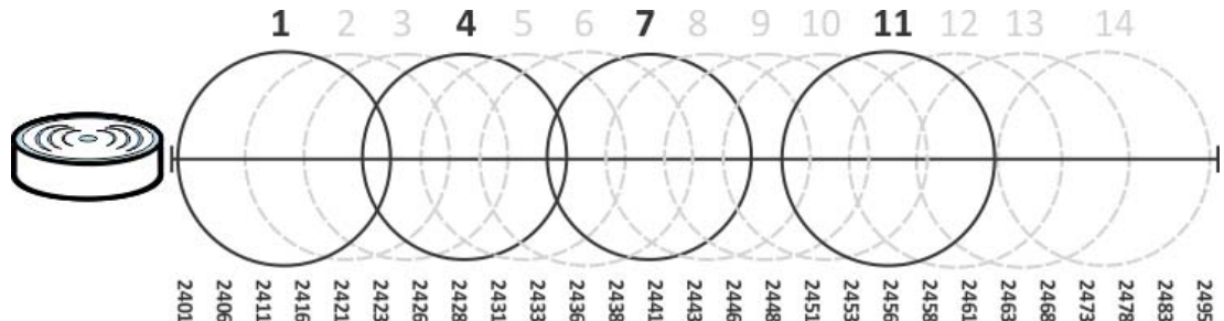
Figure 72 An Example Four-Channel Deployment
