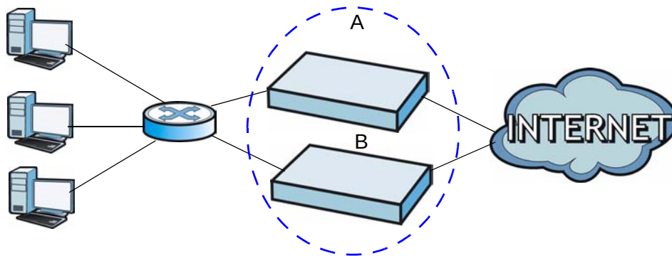
Figure 162 Virtual Router
