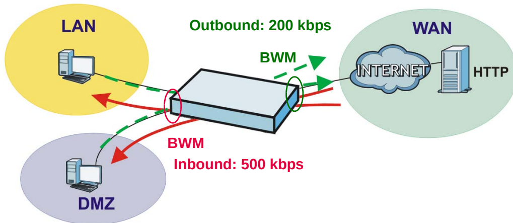
Figure 121 HTTP Any to WAN Bandwidth Management Example
