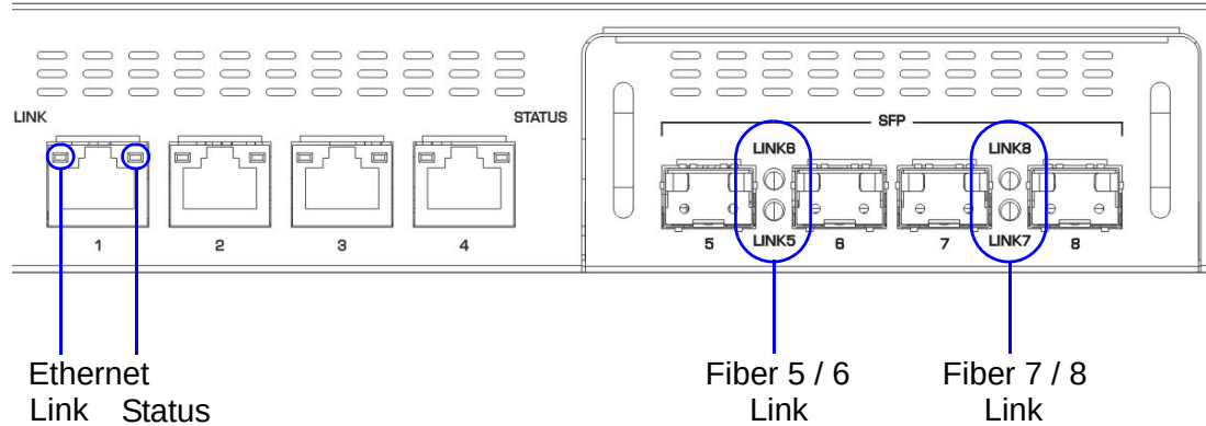
Figure 6 NXC Front Panel - Configuration 3
