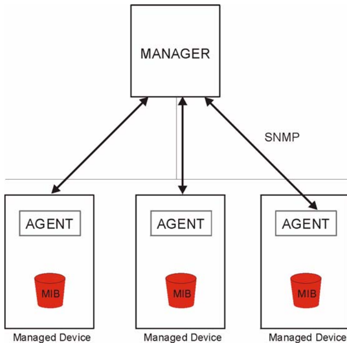
Figure 234 SNMP Management Model
