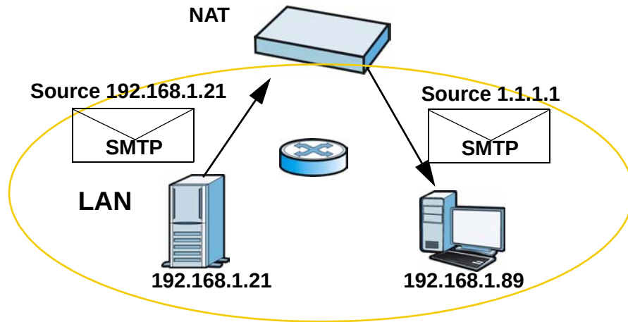
Figure 94 LAN to LAN Return Traffic
