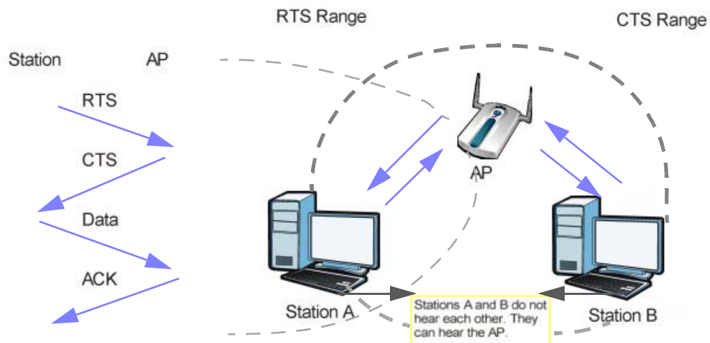
Figure 260 RTS/CTS
