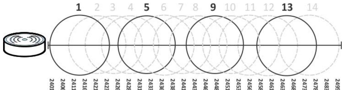
Figure 73 An Alternative Four-Channel Deployment
