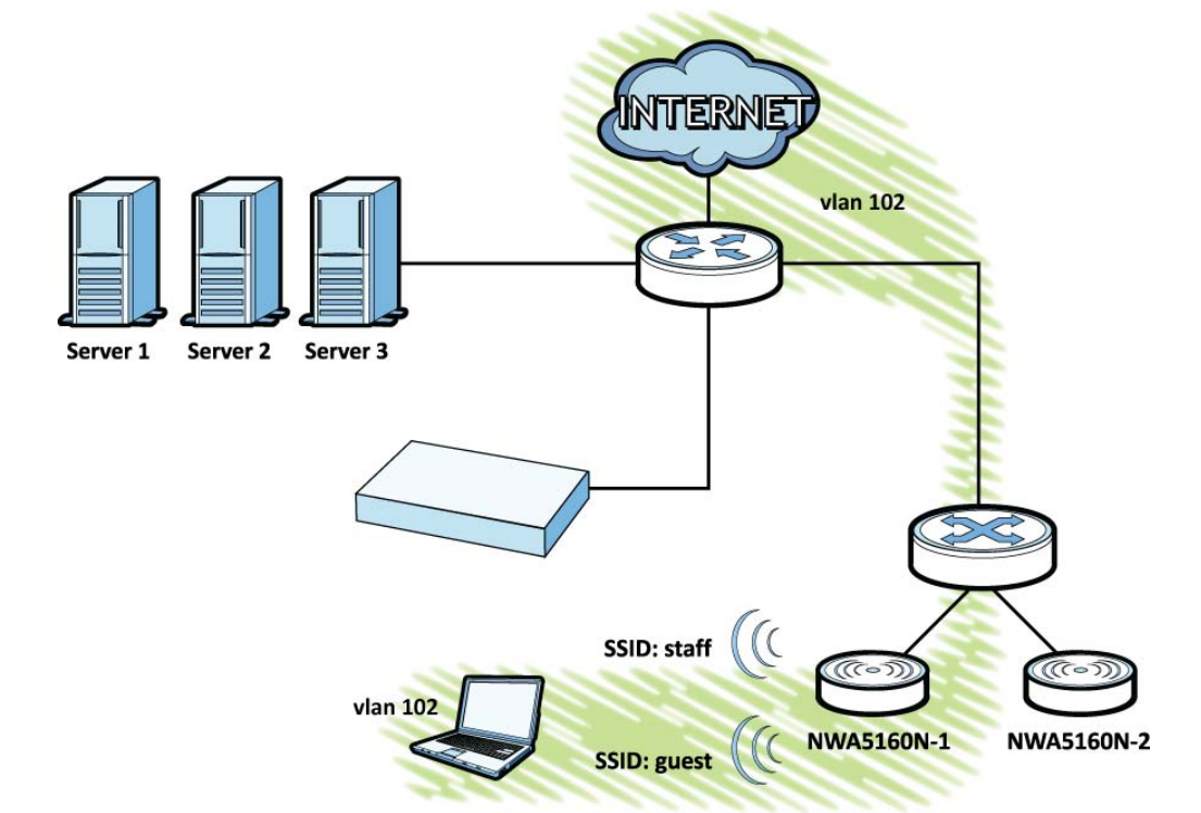
Figure 20 Tutorial Guest VLAN Example
