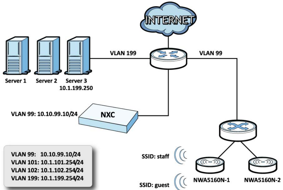
Figure 19 Tutorial Network Topology
