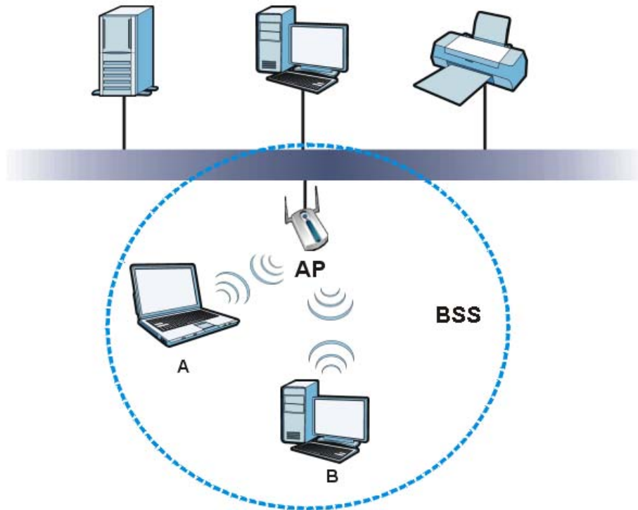
Figure 258 Basic Service Set
