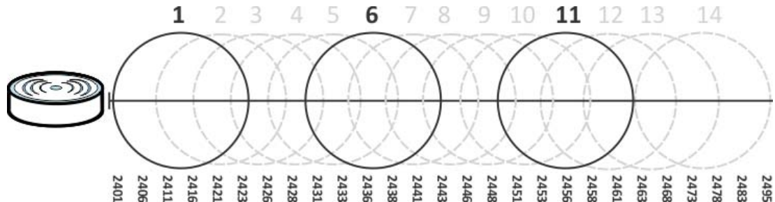
Figure 71 An Example Three-Channel Deployment
