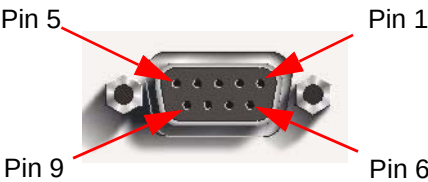
Figure 280 ALARM Connector Pin Layout
