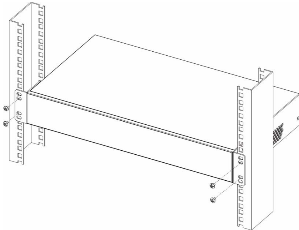
Figure 8 Rack Mounting
