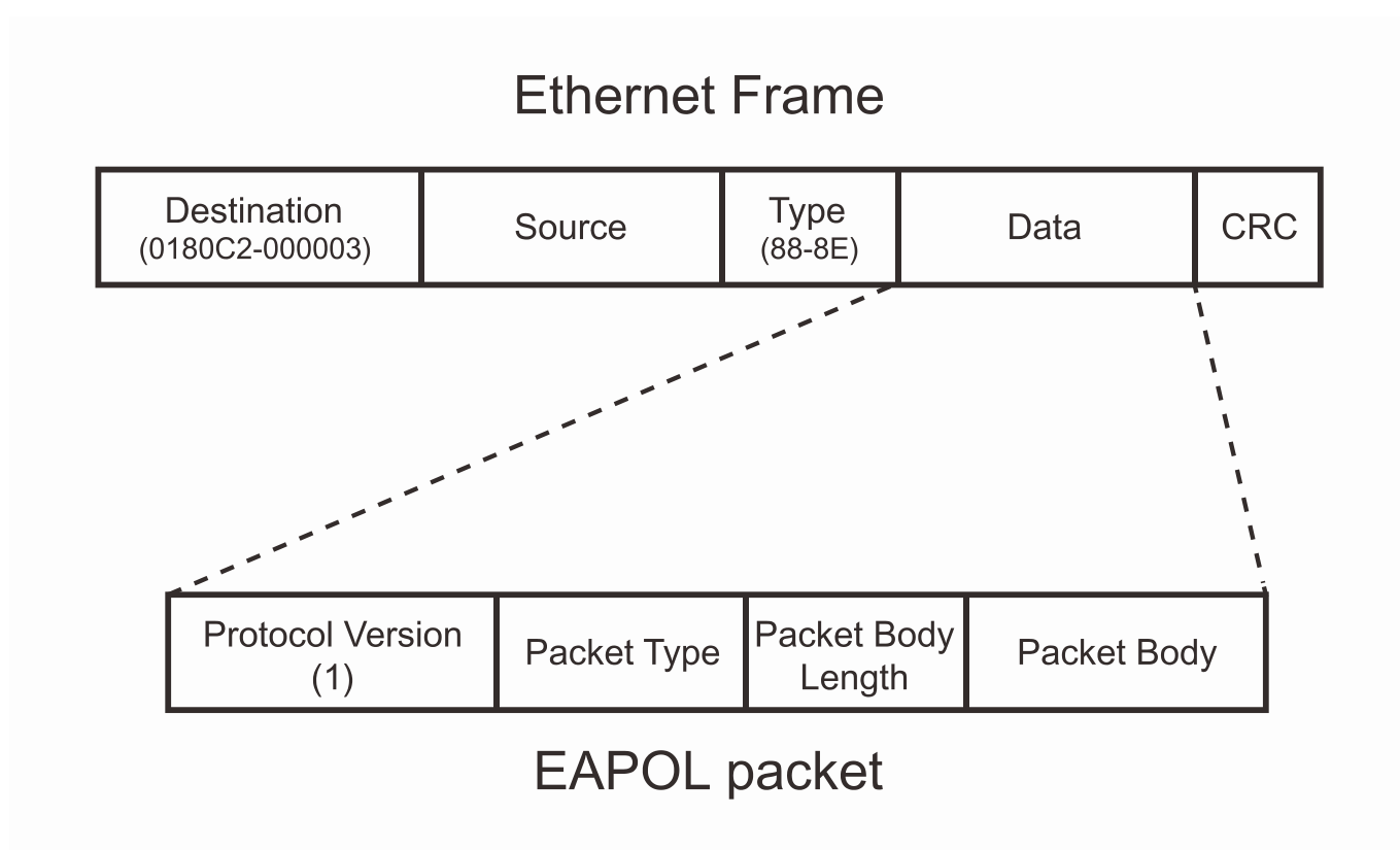
Figure 8-1 The EAPOL Packet
