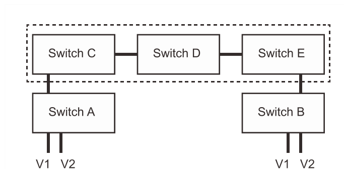
Figure 4-14 Example of VLAN Trunk
