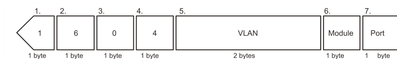
Figure 9-2 Circuit ID Sub-option Format
