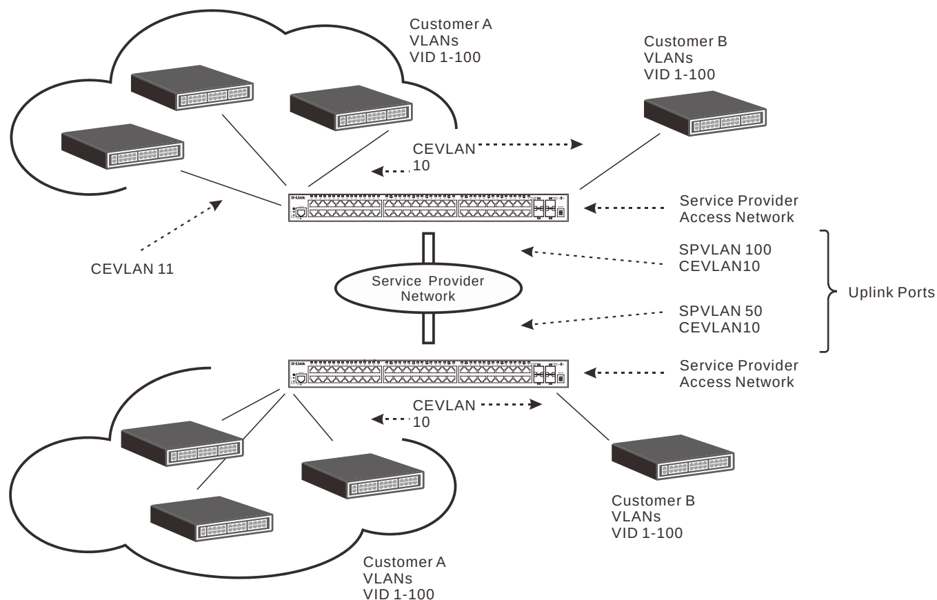
Figure 4-18 QinQ example window
