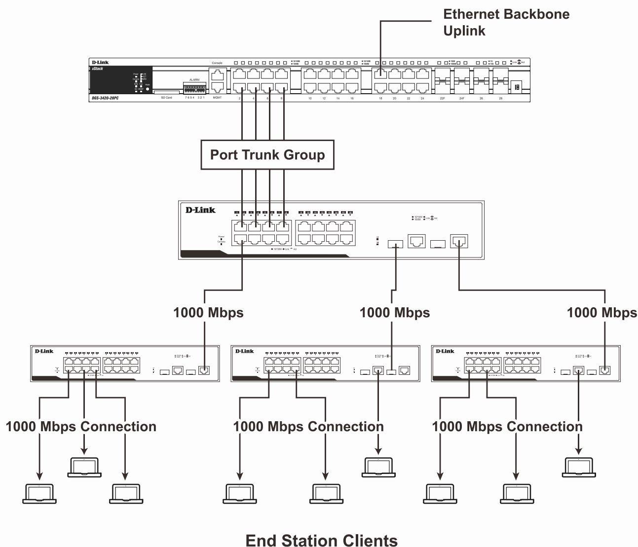
4-27 Example of Port Trunk Group
