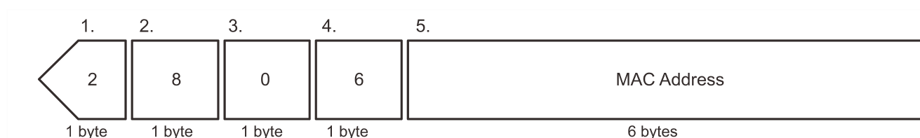
Figure 9-3 Remote ID Sub-option Format
